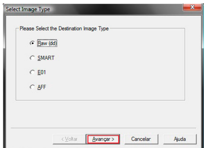
Figure 6. Select RAW
