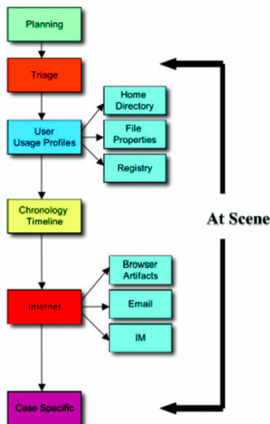
Figure 3. Investigation procedure using triage before start the extortion of information from the given devices
