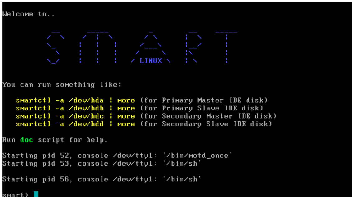
Figure 21. S.M.A.R.T. Linux
