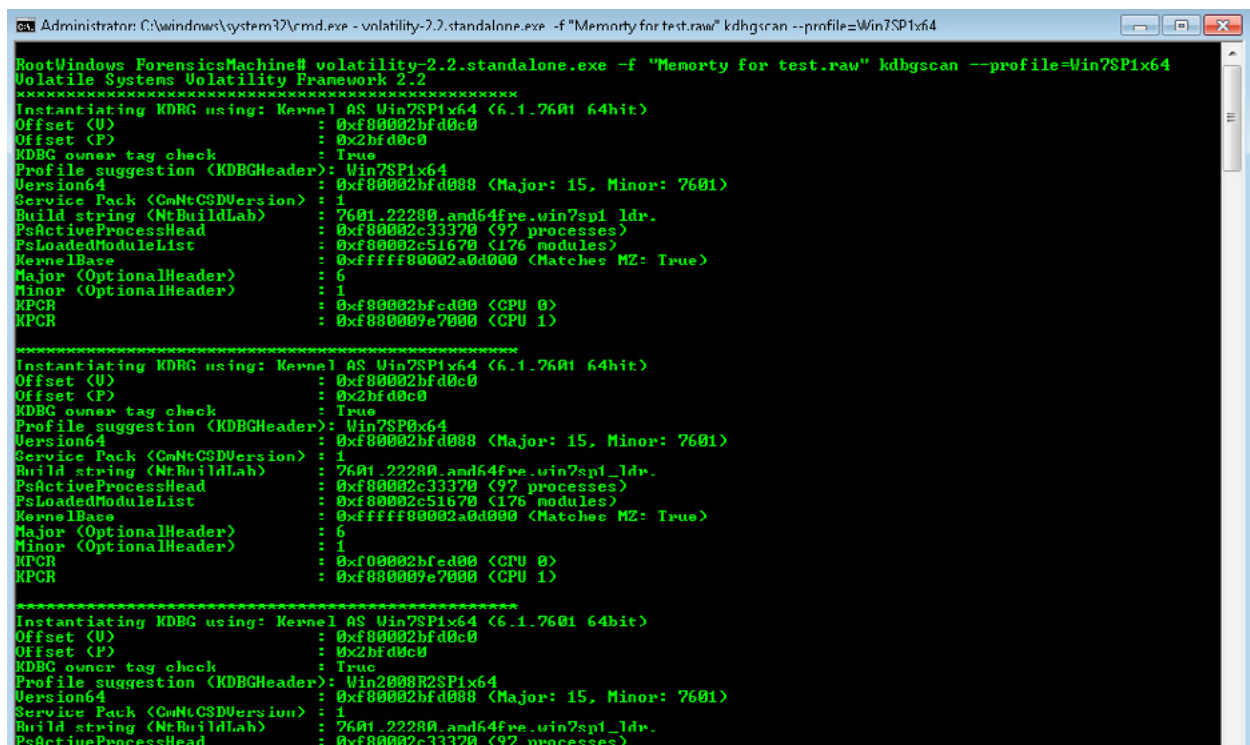
Figure 8. Using the KdgbScan
